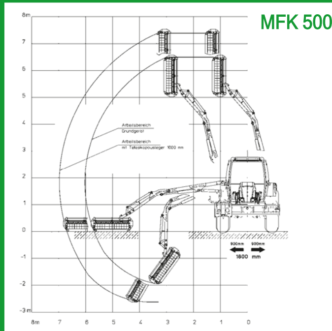
Diagram MFK 500
